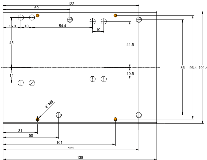
Mechanical Dimensions Bottom View
