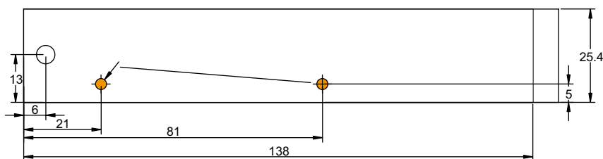
Mechanical Dimensions Side View
